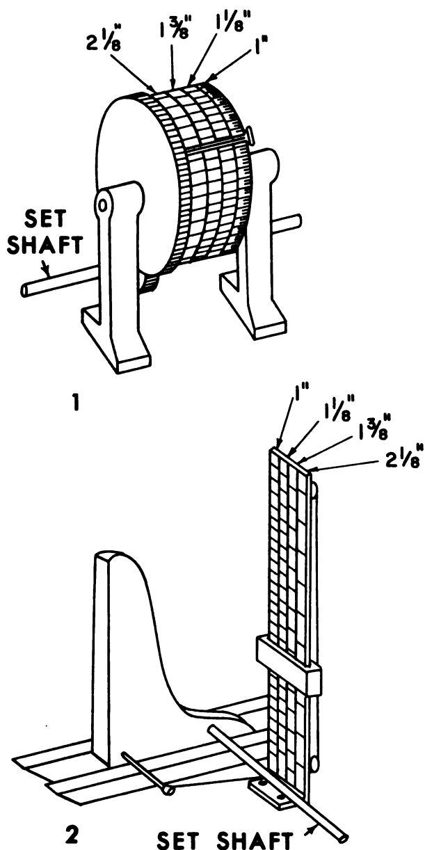
Figure 8-22. Types of indicators.
